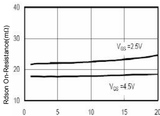
Figure 6 Drain-Source On-Resistance
