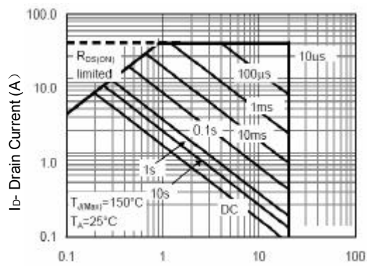
Figure 4 Safe Operation Area
