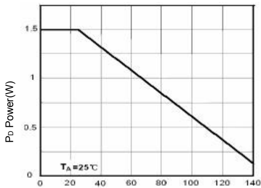
Figure 3 Power Dissipation
